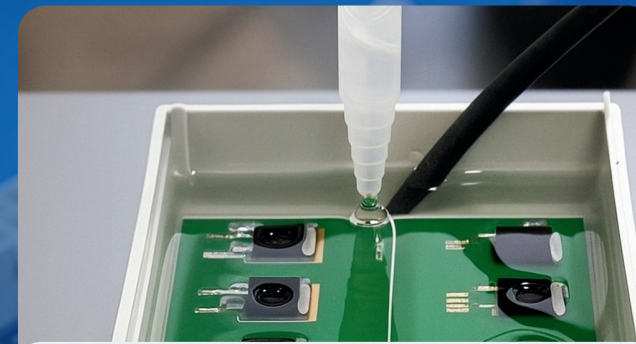
Epoxy glue
