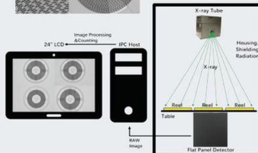
X-Ray counter
